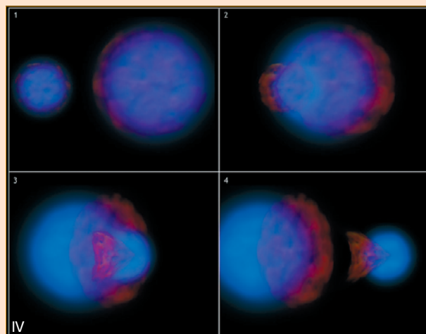
NASA/CXC/M. Weiss.
